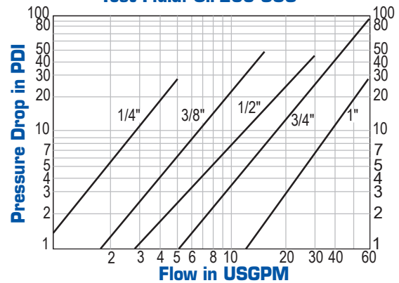
FF Series (1/4"; 3/8"; 1/2"; 3/4"; 1") Test Fluid: Oil-200 SUS
